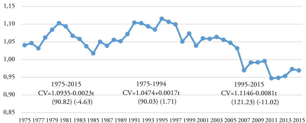
FIGURE 1. \sigma -convergence
